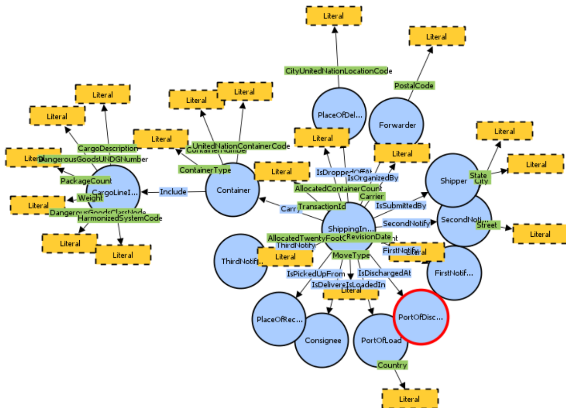
Figure 3 Shipping Instruction Ontology
