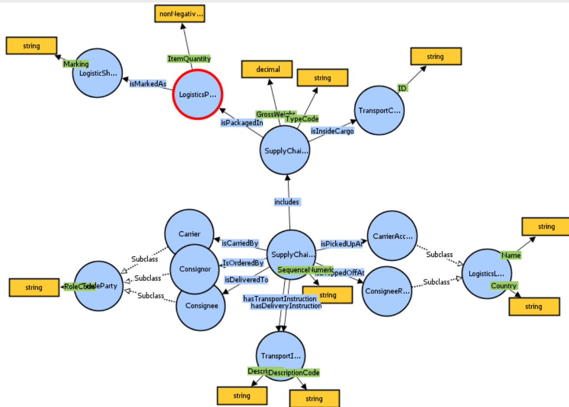
Figure 2 eCMR ontology
