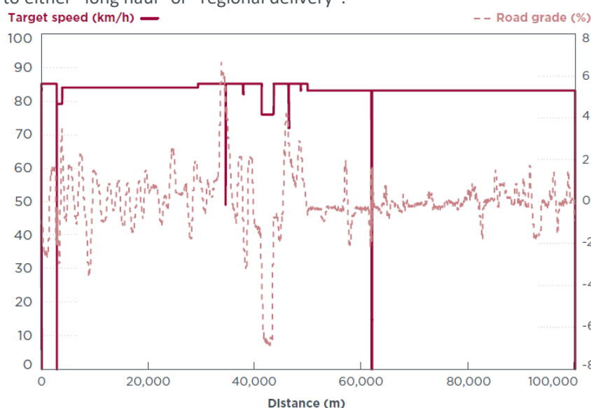
Figure 3-9: VECTO Long Haul Cycle (Delgado, Rodriguez, & Muncrief, 2017)
