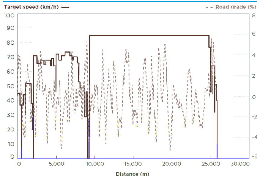
Figure 3-10: VECTO Regional Delivery Cycle (Delgado, Rodriguez, & Muncrief, 2017)
