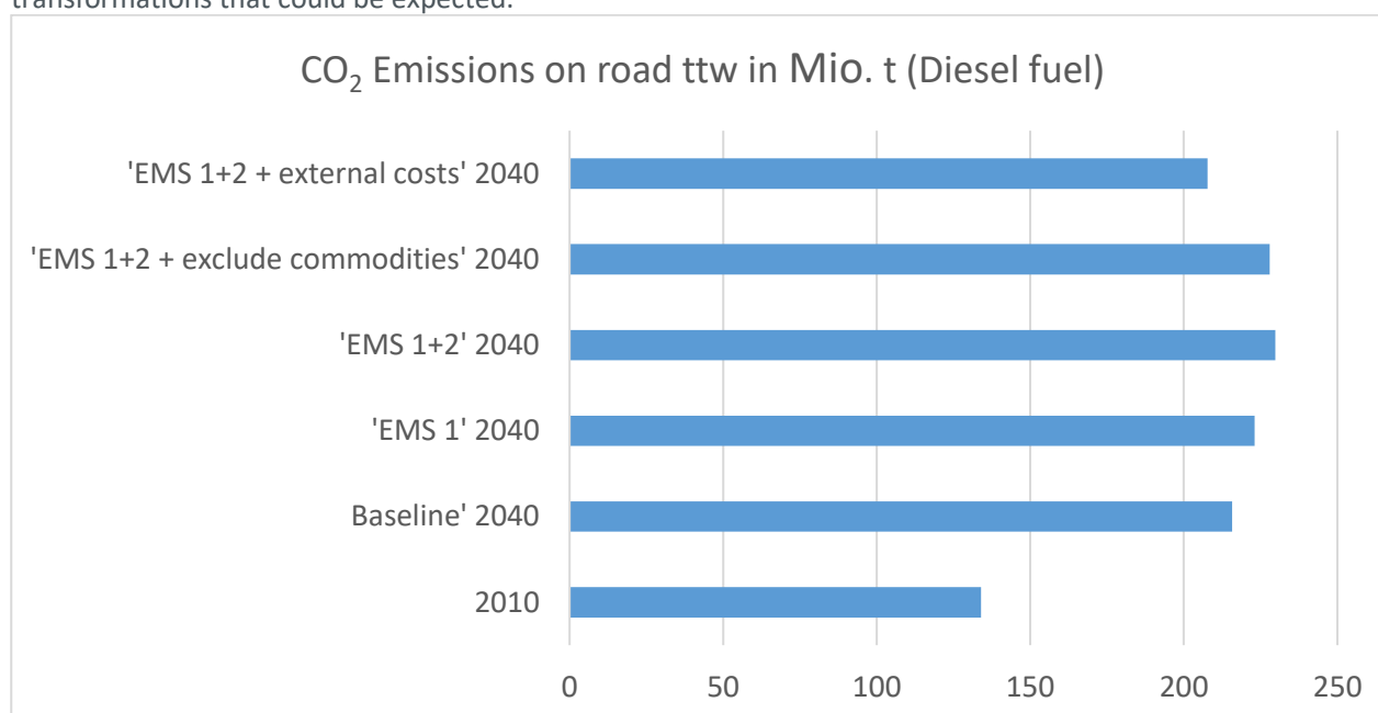
Figure 3-3: Impact on CO 2 emissions on road transport (ttw: tank-to-wheel)
