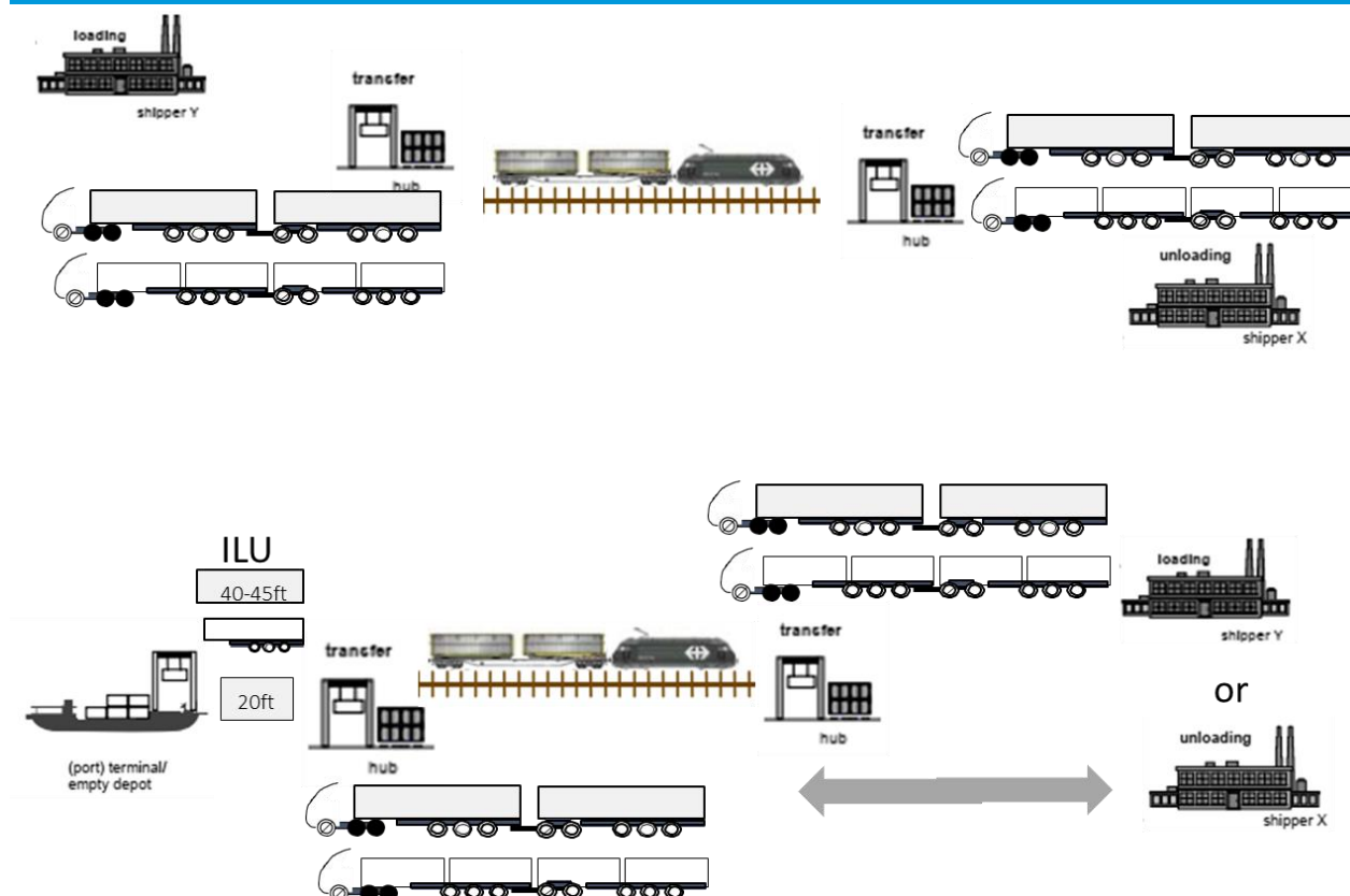
Figure 3-6: Intermodal transport chain – use of EMS 2 for national and international transports
