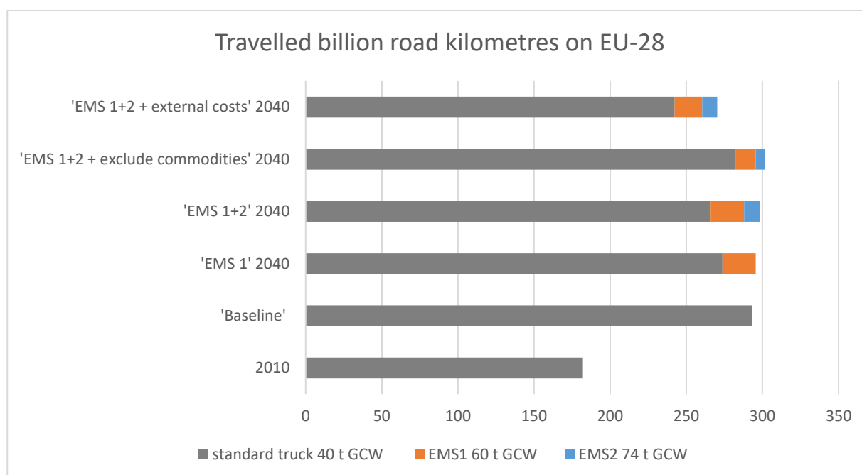
Figure 3-2: Travelled road kilometres of heavy trucks (40 t GCW, EMS 1, EMS 2) for all scenarios
