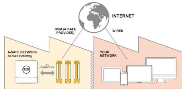
Figure 9 A-SAFE Network Architecture with RackEye Devices
